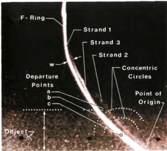
Plate 26: Photograph of braided F-ring exposed to reveal a large coupled object.
