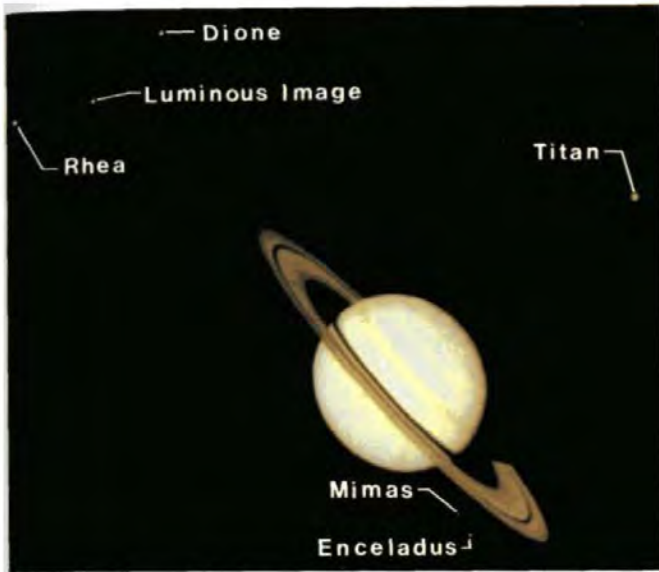
Plate 11: Saturn, five Saturnian moons and an unexpected luminous image.
