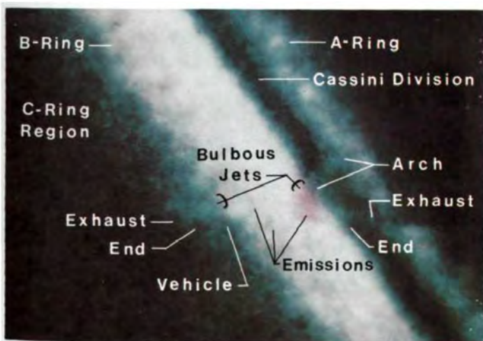
Plate 9: Partially developed ring system exhibiting a transversely positioned cylindrical vehicle in the B-ring.
