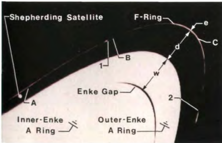
23: Non-uniformly luminescent F-ring in positional relation to A-ring components and a shepherding satellite.
