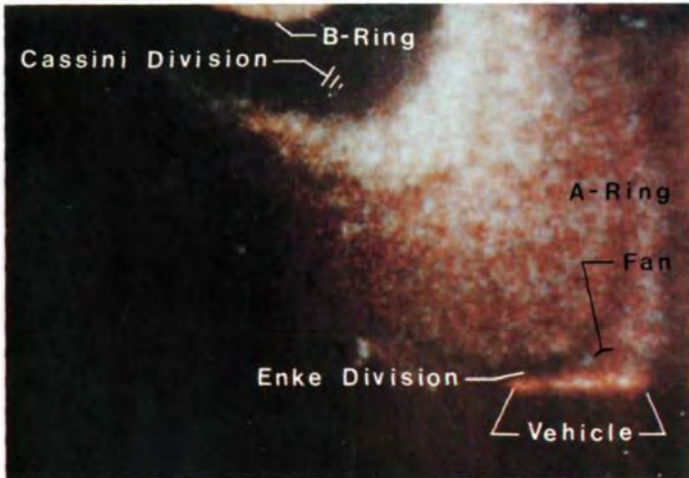
Plate 7: Formation of the Enke division.
