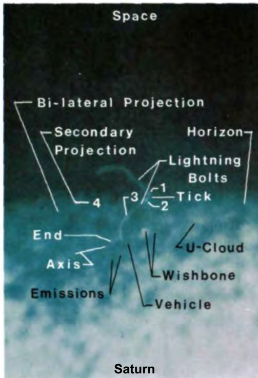
Plate 16: Two lightning bolts appear in and above Saturn's cloud tops. Photograph is an enlargement of Plate 14 in the area labeled "lightning location".
