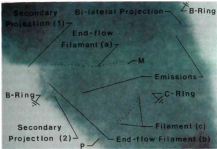
Plate 22: B-ring emissions become C-ring constituents.
