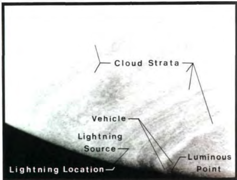
Plate 14: Sector of southern hemisphere of Saturn showing cloud strata, a luminous point, location of a lightning source and a slender vehicle. (Non-optimum exposure for overall picture favors the dark region at planet horizon).
