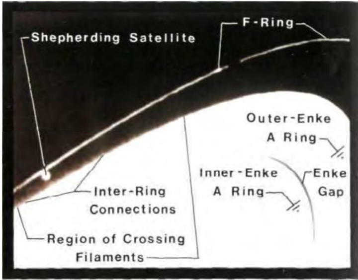
Plate 25: Non-uniformly luminescent F-ring of Plate 23 exposed to reveal inter-connections between the F-ring and A-ring outer edge.
