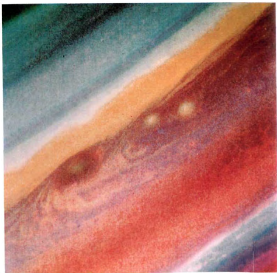
Frontispiece: A spectacular pattern in Saturn's atmosphere masks the presence of awesome power.
