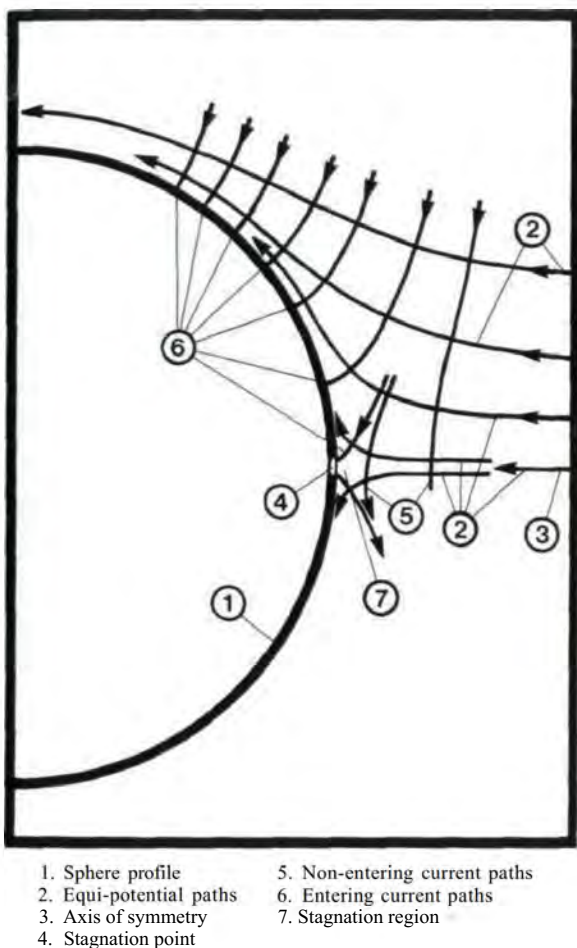
Plate 41: Network of electrical current and equi-potential paths calculated for a sphere in ideal flow.
