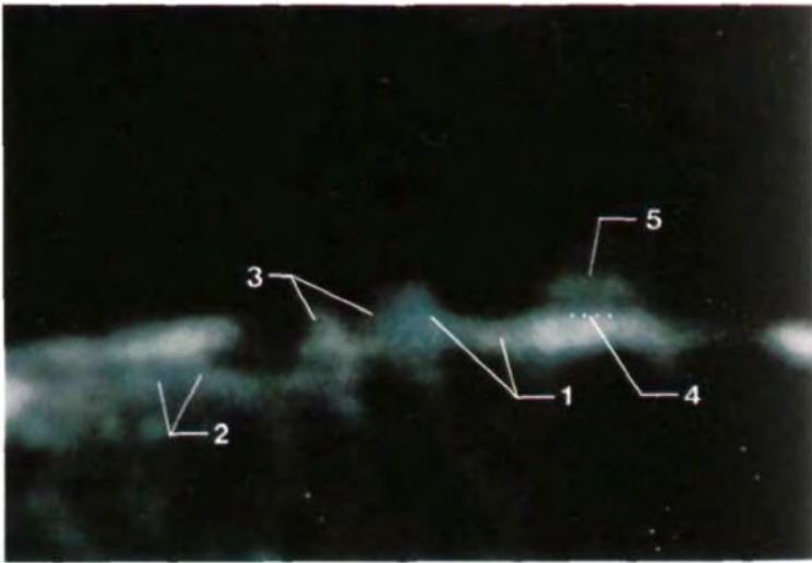
Plate 33: Dione's narrow-band illuminated topography showing various types of emissions.
