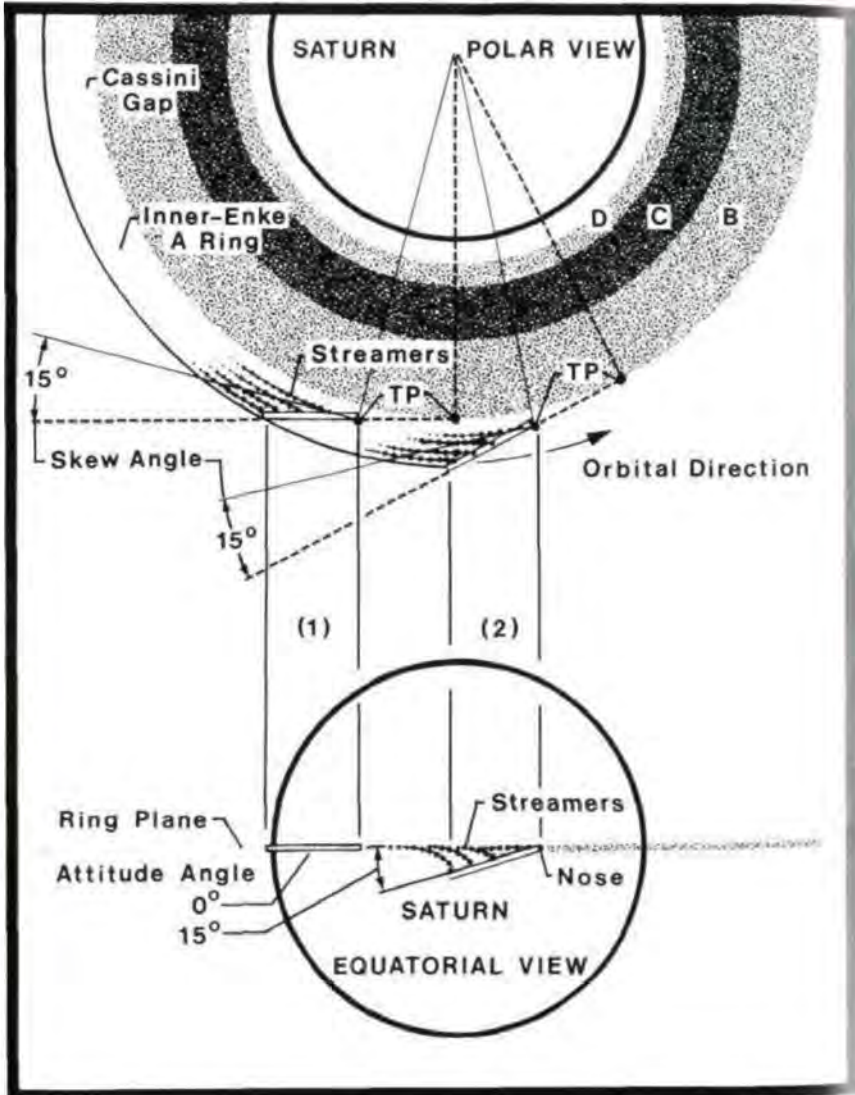
Plate 28: A simplified electromagnetic vehicle in different attitude angles for two orbital positions during formation of the inner-Enke A-ring.
