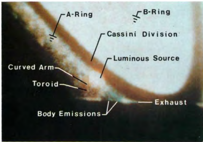
Plate 6: A slender vehicle forms an A-ring trail which includes a luminous source.
