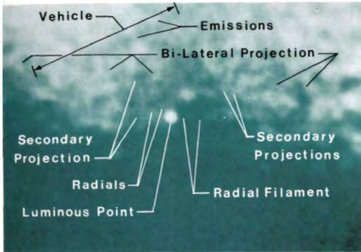
Plate 15: Luminous point of Plate 14 essentially is an are light whose apparent power source is a remote vehicle capable of generating paths carrying electricity.
