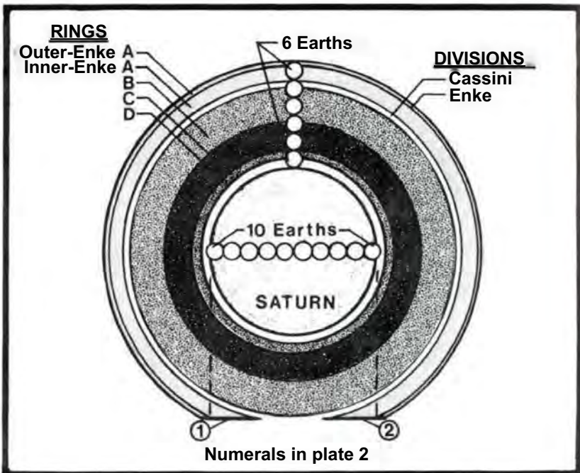
Plate 4: Conceptualization of the incomplete A-ring in a polar view of Saturn's northern hemisphere, using Earth as a comparable reference measure.
