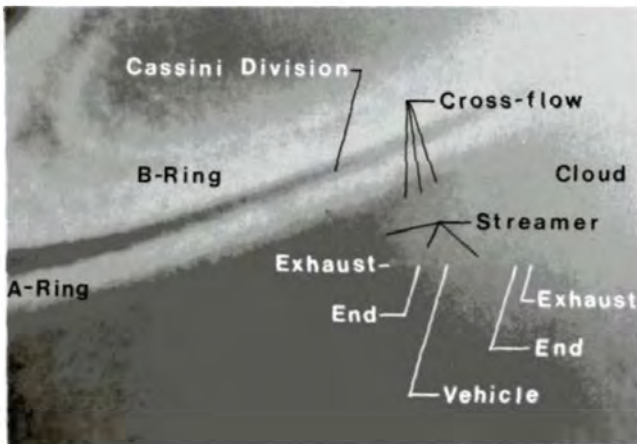
Plate 10: Emitting vehicle stationed outside the A-ring encompasses the F-ring location.
