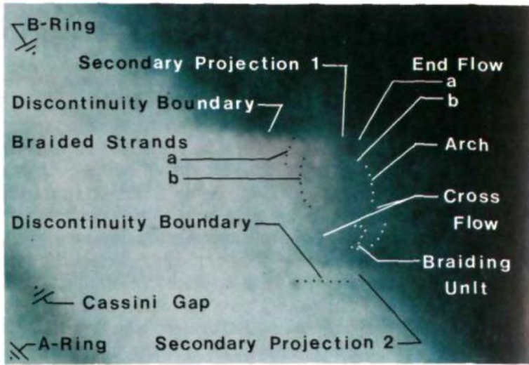
Plate 21: Braided strands, a braiding unit and cross flow between discontinuity boundaries at the B-ring inner edge.
