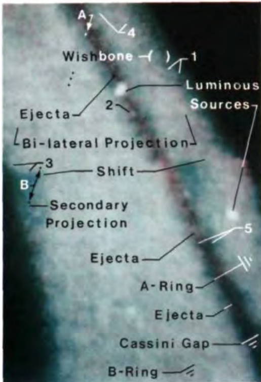
Plate 18: Luminous sources provide clue to presence of electromagnetic vehicles as a causative mechanism for a filled Cassini gap and an apparent ring shift.
