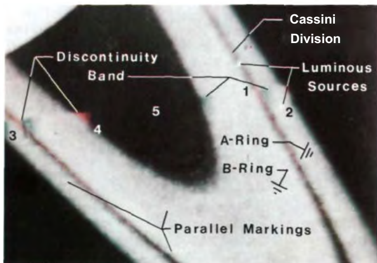
Plate 17: A colorful, large-scale narrow-band disruption in Saturn's rings extending across the entire ring system.
