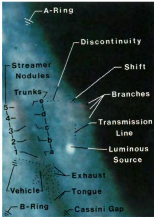
Plate 19: Vehicle and ejecta in the Cassini gap in relation to an A-ring discontinuity, apparent ring shift and a luminous source.
