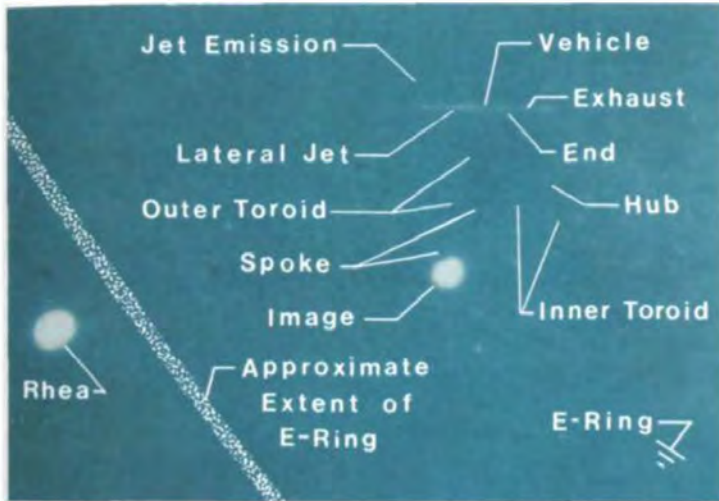
Plate 13: Enlargement of luminous image revealing a nearby slender vehicle within the E-ring.
