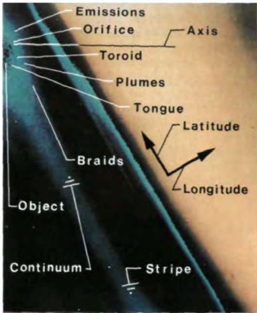
Plate 29: A dark blue latitudinal stripe in Saturn's atmosphere emanates from an object identifiable as a probable electromagnetic vehicle component.
