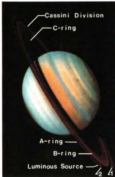
Plate 3: A luminous source appears in the A-ring of Saturn.
